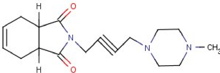
AM-5: 2-[4-(4-methylpiperazin-1-yl)but-2-yn-1-yl]-2,3,3a,4,7,7a-hexahydro-1H-isoindole-1,3-dione
